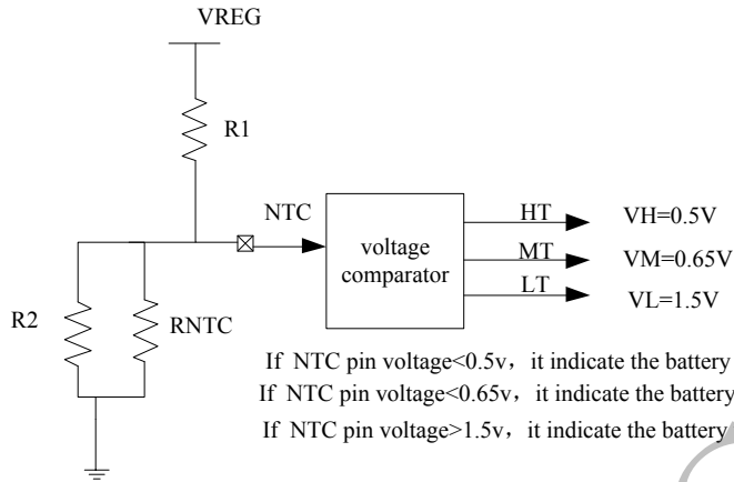
Fig 6 Battery NTC threshold
