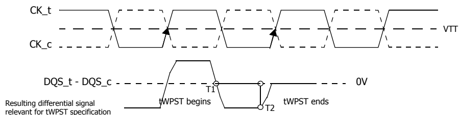
Figure. Method for Caculating tWPRE Transitions and Endpoints
