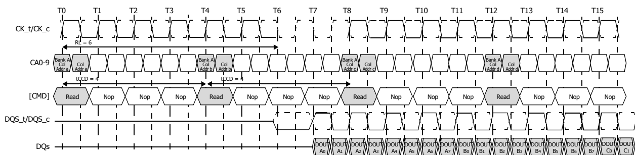
Figure. Seamless Burst READ: RL = 6, BL = 8, tCCD = 4
