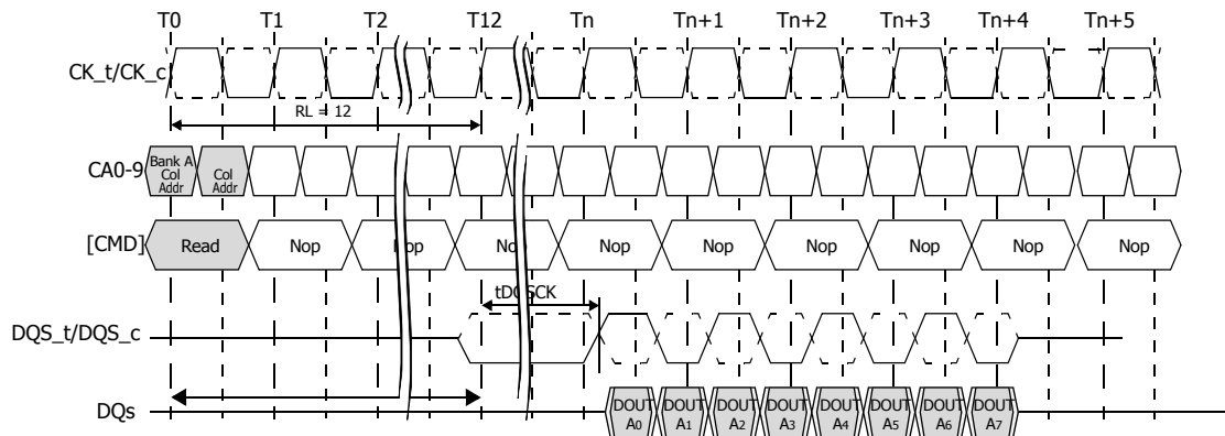
Figure. Burst Read : RL=12, BL=8, tDQSK < tCK
