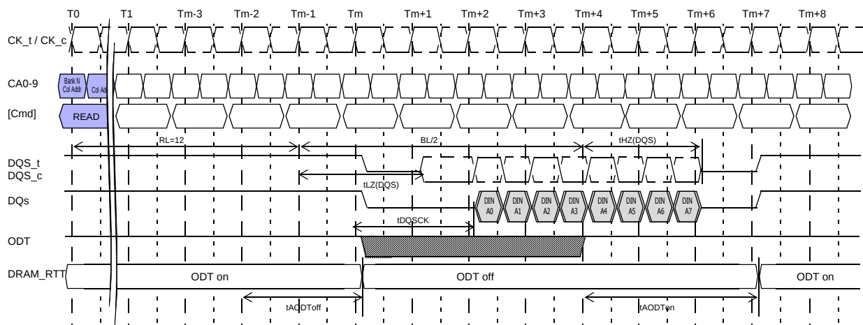
Figure. Automatic ODT Timing During READ Operation Example for RL=m
